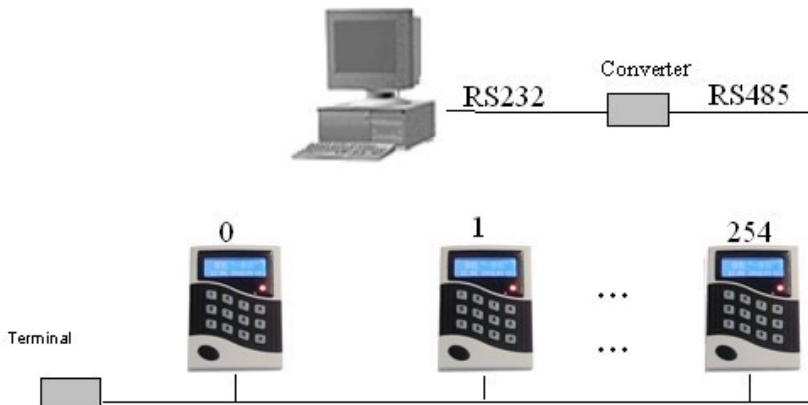
Figure 2-3 RS485 multiple networking
